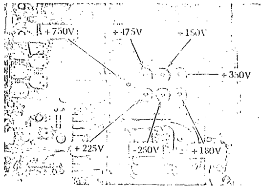
Fig. 2. Type 517 Oscilloscope power supply test points.
