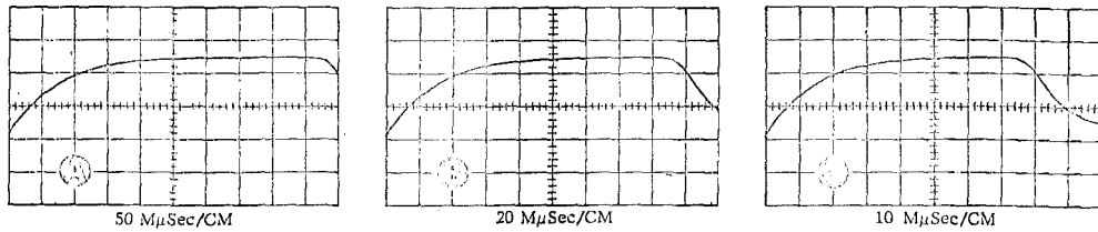
Fig. 11. Waveforms obtained when the +GATE is adjusted properly for the respective sweep rates.
